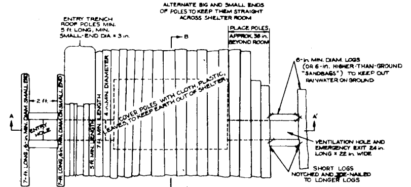
ROOF POLES MINIMUM 7-ft LONG, 4-in. MINIMUM DIAMETER LAID ABOUT 2 ft. PAST EACH FT. OF SHELTER ROOM. PLAN VIEW OF TOP OF SHELTER SHOWING PLACEMENT OF POLES FOR ROOF (EARTH FILL NOT SHOWN)
