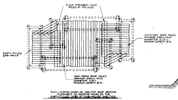
Fig. A.6. Aboveground, Crib-Walled Shelter.
