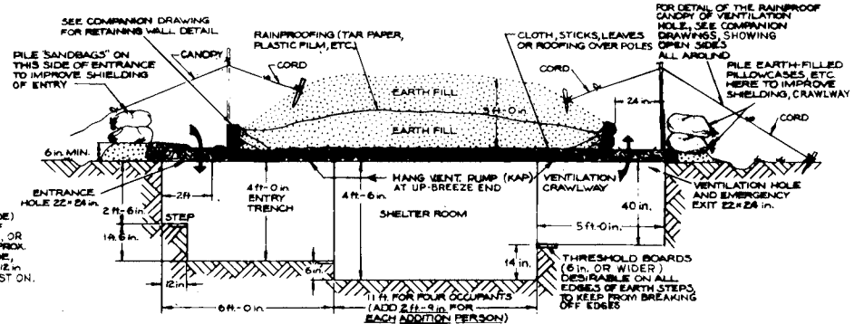
VIEW A-A, CROSS SECTION THROUGH LENGTH OF TRENCH SHELTER
