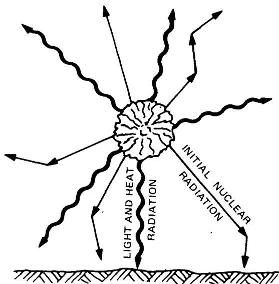
Fig. 1.4. An air burst. The fireball does not touch the ground. No crater. An air burst produces only extremely small radioactive particles—so small that they are airborne for days to years unless brought to earth by rain or snow. Wet deposition of fallout from both surface and air bursts can result in “hot spots” at, close to, or far from ground zero. However, such “hot spots” from air bursts are much less dangerous than the fallout produced by the surface or near-surface bursting of the same weapons.
