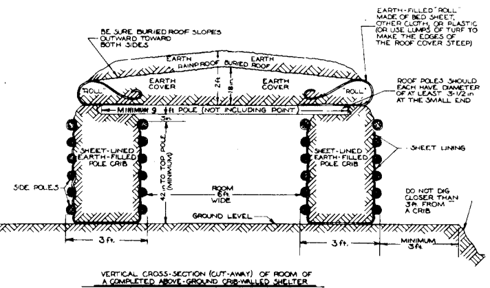
Fig. A.6. Aboveground, Crib-Walled Shelter.
