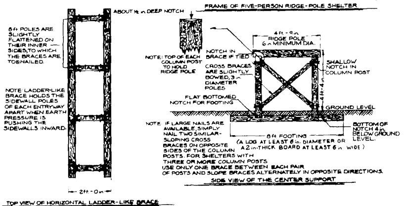
Fig. A.5. Aboveground, Ridgpole Shelter.
