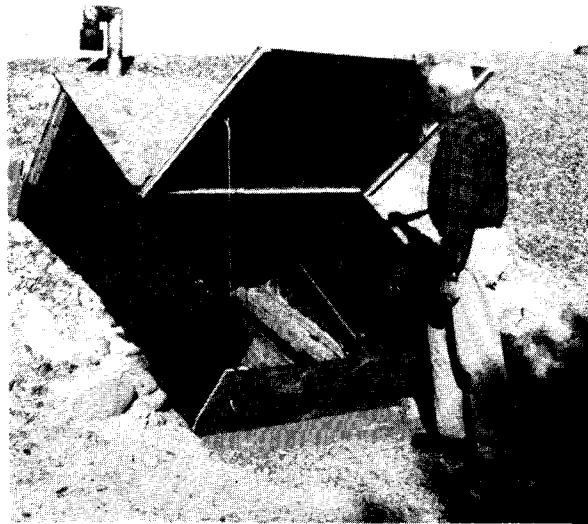
Fig. F.5. A Quickly Installable, 4-Piece Entryway Cover That Provides Easy Access and a Large, Protected Ventilation Opening.
