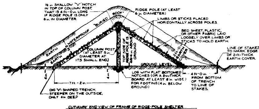
Fig. A.5. Aboveground, Ridgpole Shelter.
