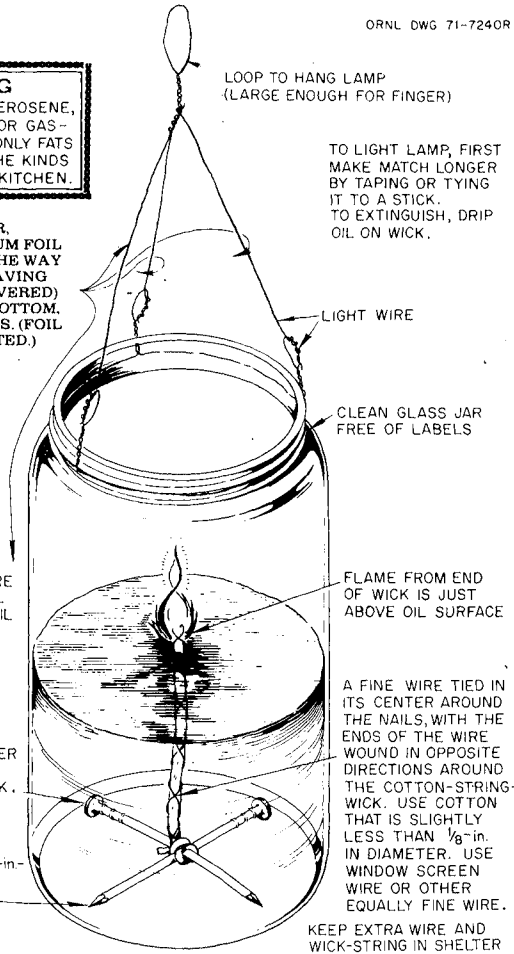
WIRE-STIFFENED-WICK LAMP
