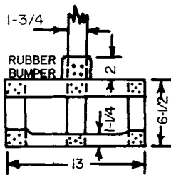
Fig. 15. Piston Rod Handle Made of 3/4 x 1-3/4-in. Boards.
