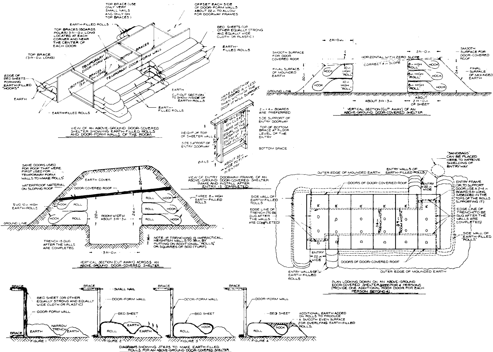
Fig. A.4. Aboveground, Door-Covered Shelter.
