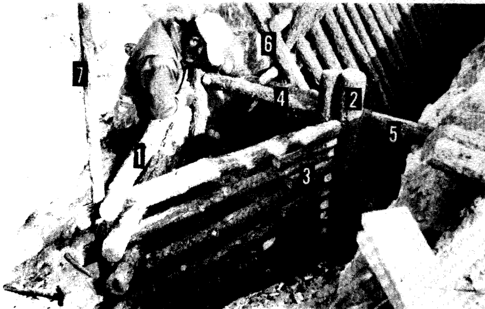
Fig. D.10. Uncompleted lower section of a vertical triangular entry.
