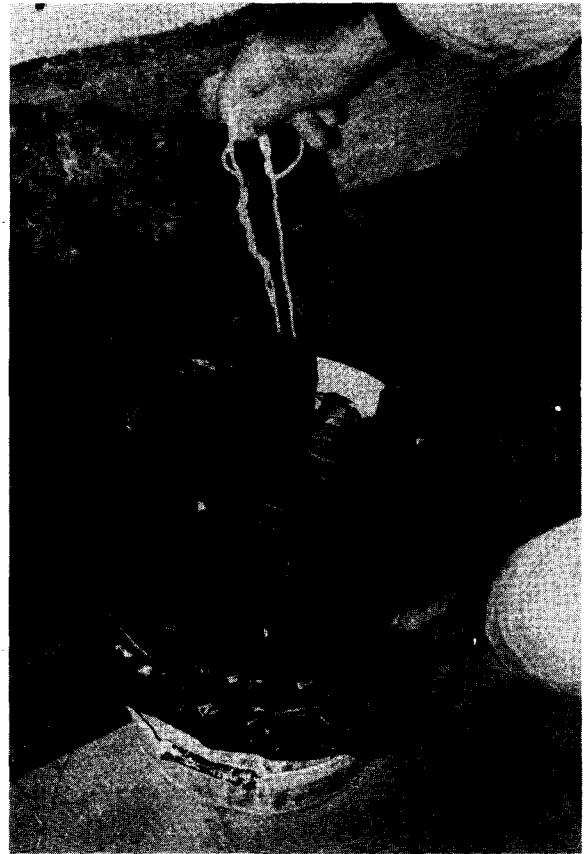
Fig. 12.1. A 5-gallon paint can used for a hose-vented toilet-can, with a plastic trash bag for its removable liner.
